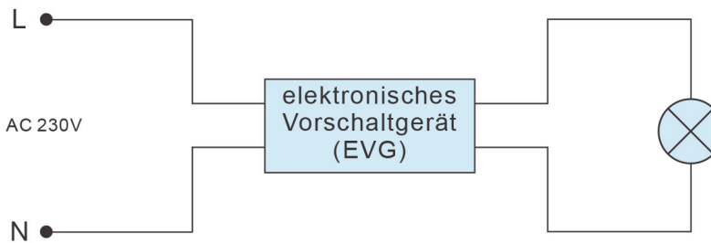
HQI/HQL Lampe
